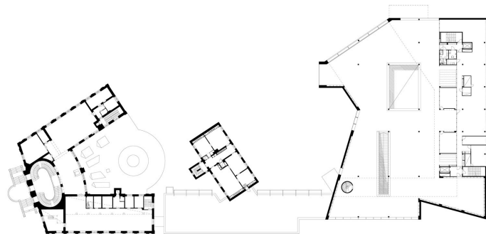
Turku Main Library_JKMM Architects_2007_ alaprajz 1. emelet
